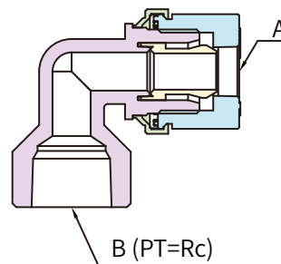
FEMALE ELBOW
