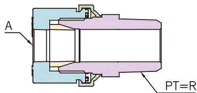
MALE CONNECTOR (FERRULE TYPE)
