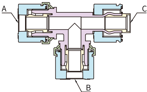
UNION TEE ADAPTOR (SLEEVE & NUT SET)
