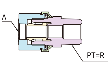
MALE CONNECTOR
