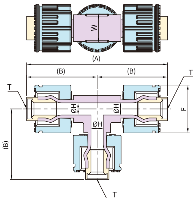
▲ Sleeve & Nut Set
