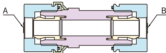
PANEL MOUNT REDUCING UNION CONNECTOR
