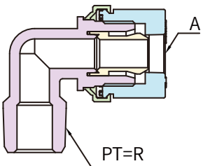
MALE ELBOW
