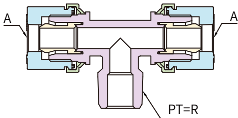
MALE TEE
