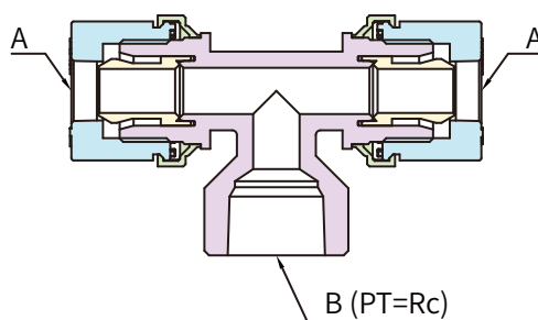
FEMALE TEE
