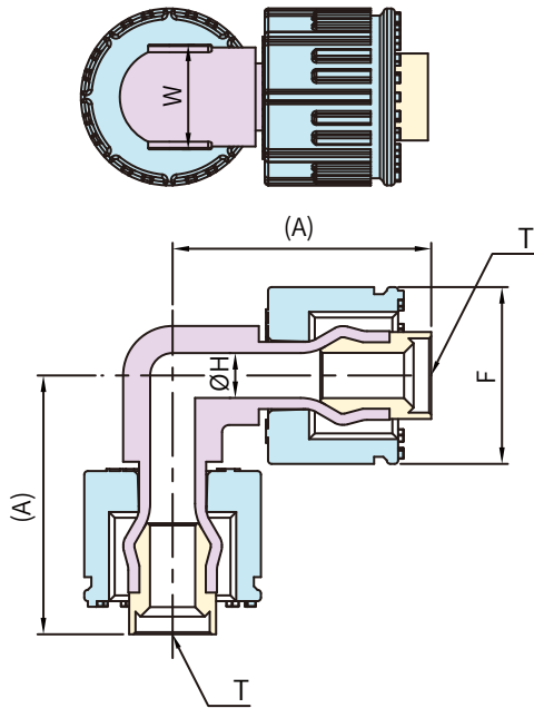
▲ Sleeve & Nut Set
